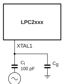
Fig 25. Slave mode operation of the on-chip oscillator
