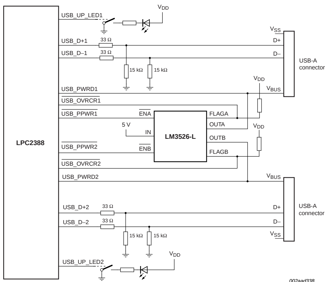
Fig 24. LPC2388 USB OTG port configuration: USB port 1 host, USB port 2 host
