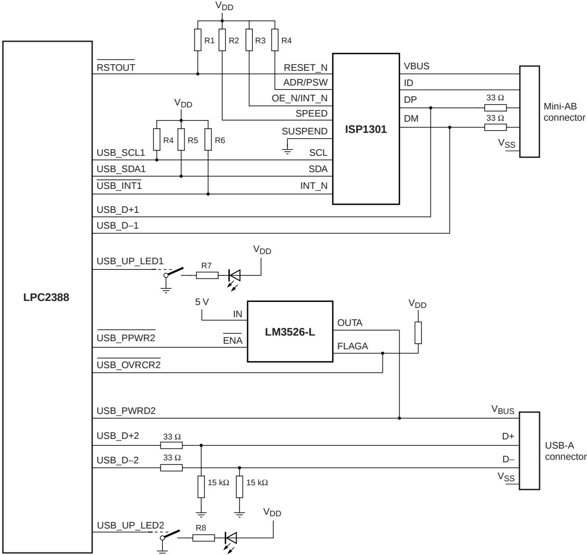
Fig 21. LPC2388 USB OTG port configuration: USB port 1 OTG dual-role device, USB port 2 host
