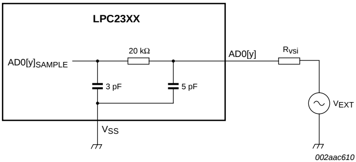
Fig 18. Suggested ADC interface - LPC2388 AD0[y] pin
