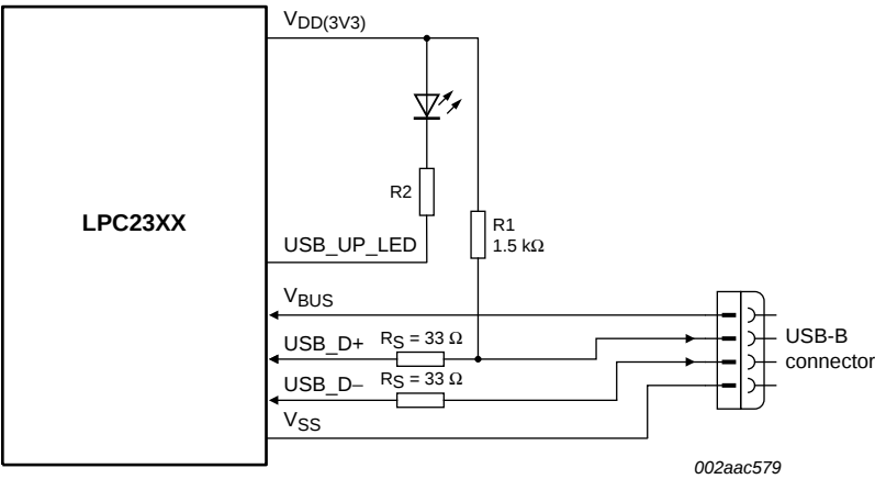
Fig 20. LPC2388 USB interface on a bus-powered device (applies to USB ports 1 and 2)
