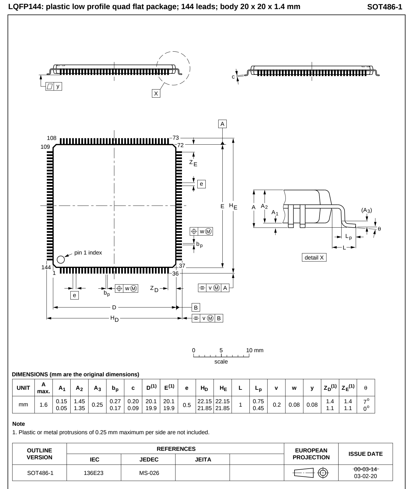
Fig 30. Package outline SOT486-1 (LQFP144)
