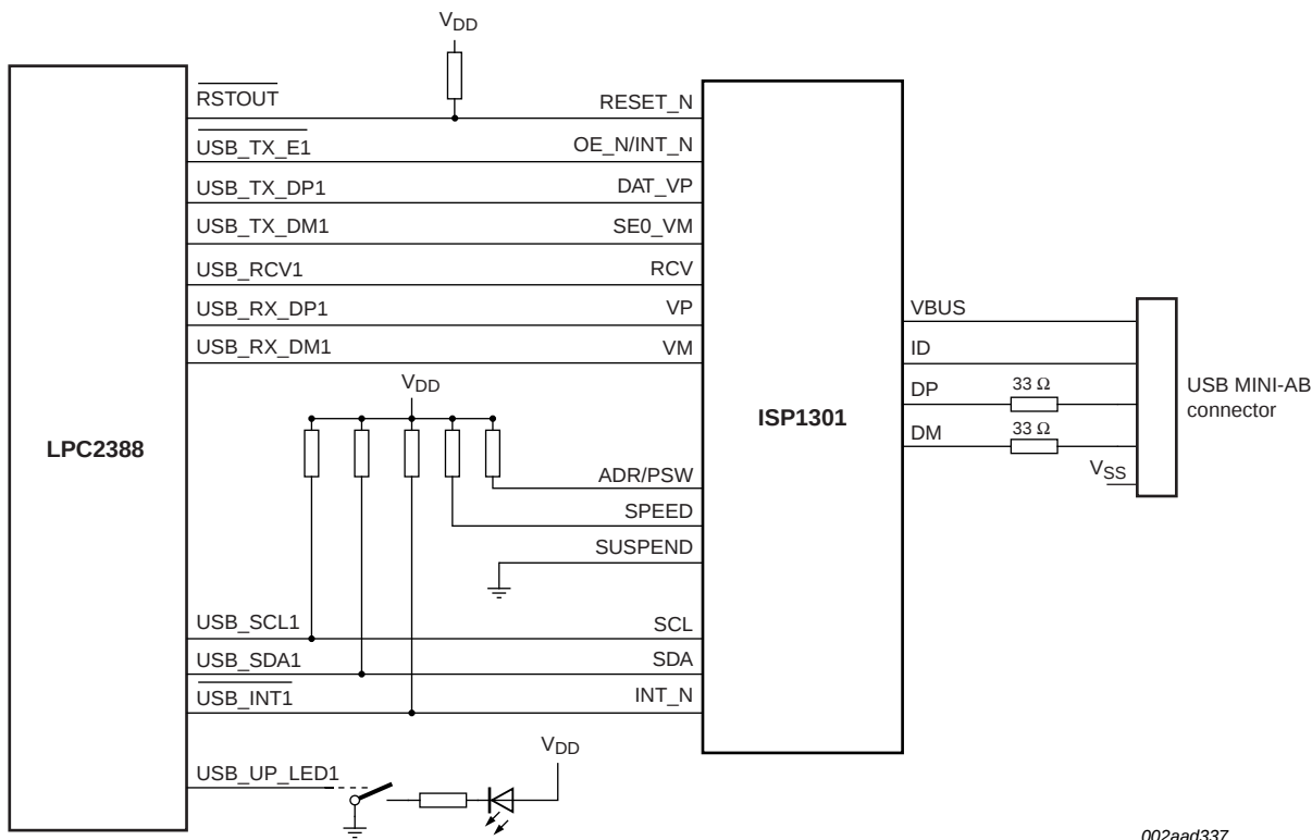
Fig 22. LPC2388 USB OTG port configuration: VP_VM mode
